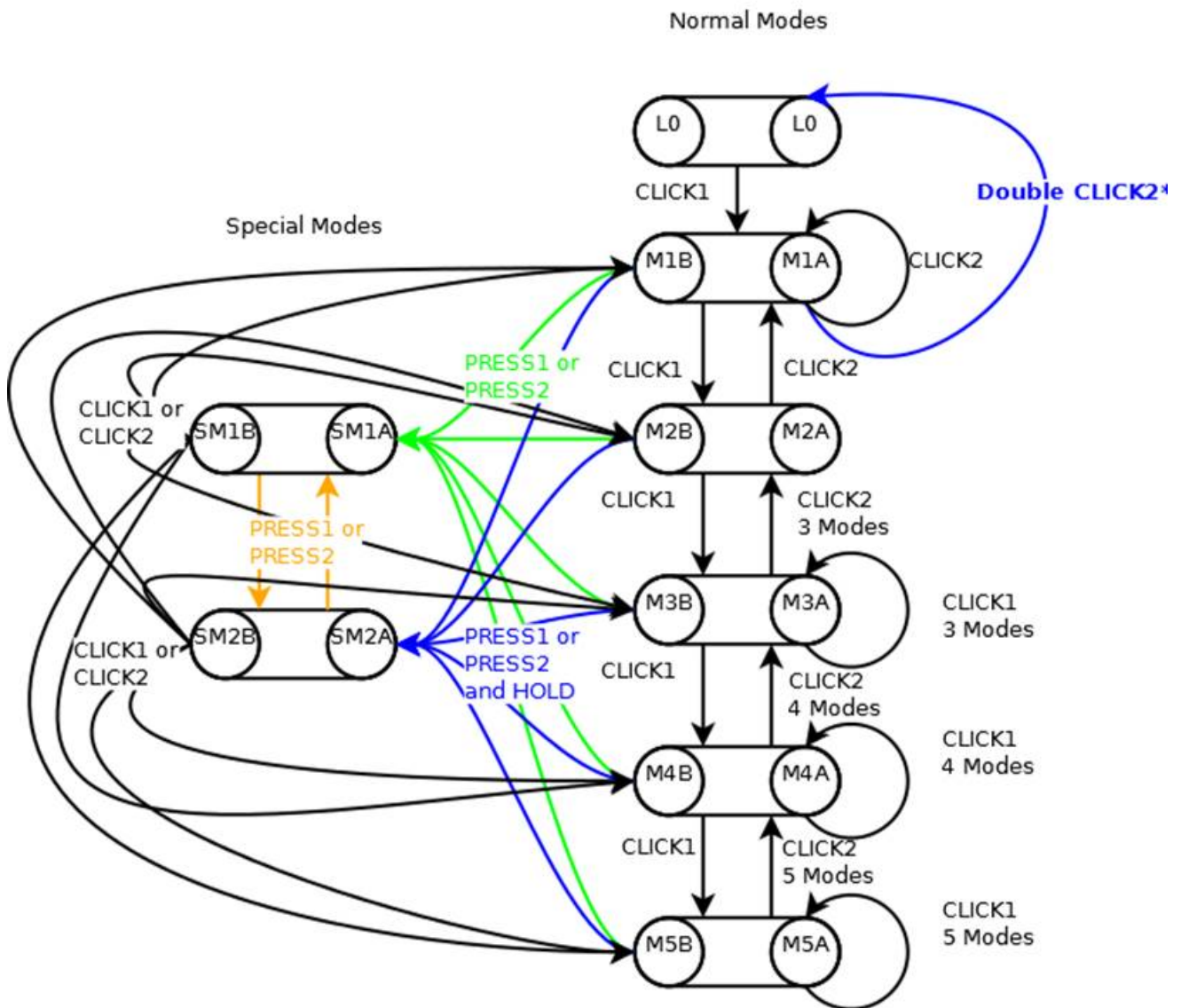
UIC3 Flow Diagram
