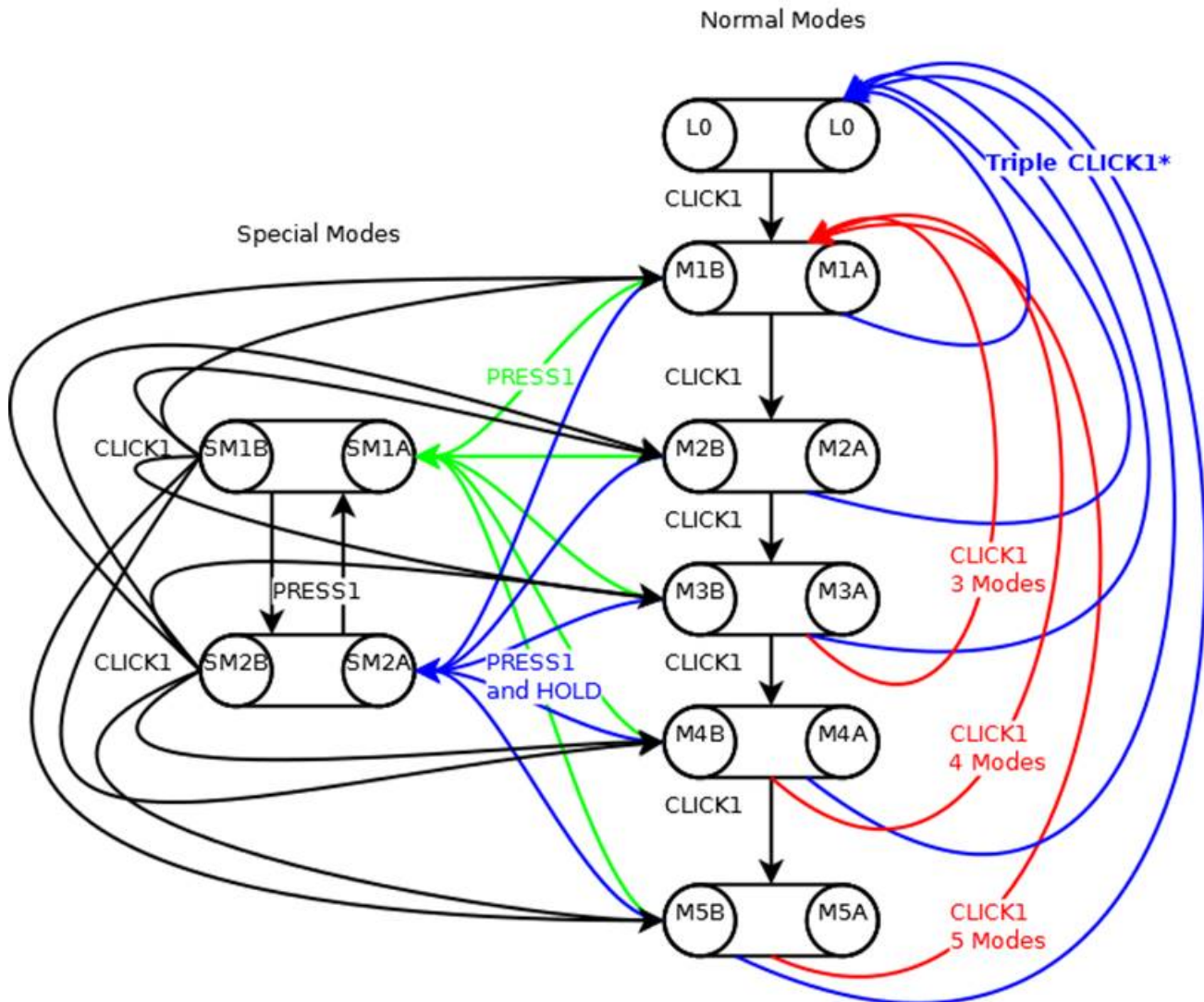
UIC2W Flow Diagram
